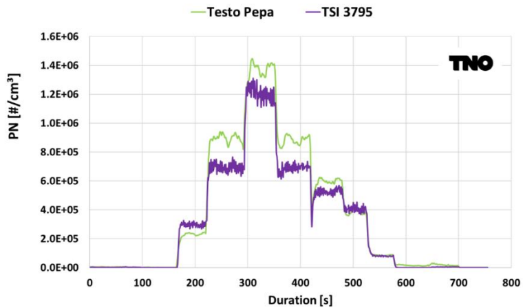
Figure 25: PN emissions measured with two different mobile PN-testers at low idle speed of a Peugeot Partner diesel Euro 6b with different DPF bypass exhaust flows (2 nd measuring campaign).
