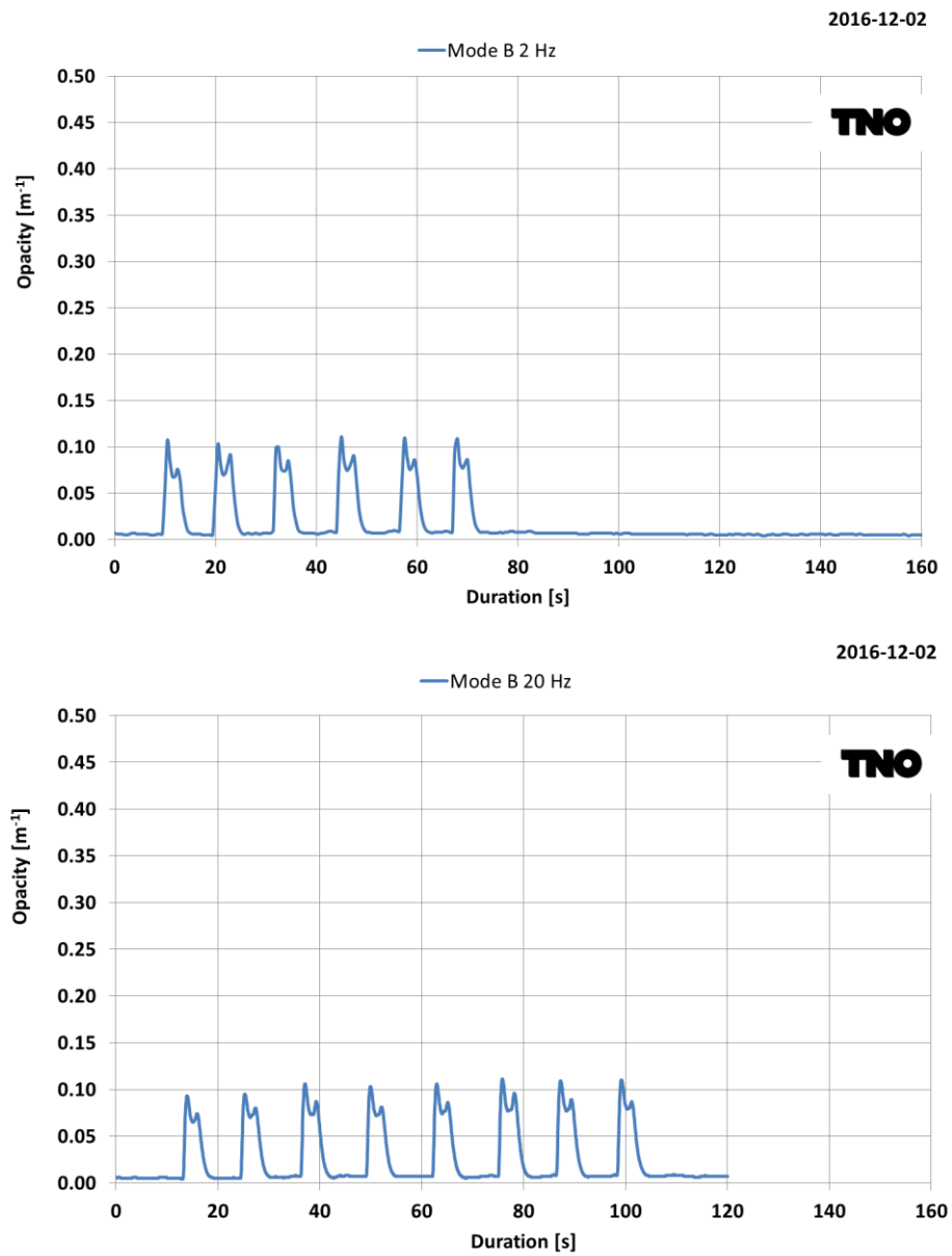
Figure 9: Free acceleration smoke emission test results (Mode B) of a Ford Fiesta Euro 6 diesel vehicle with a small DPF leakage with different sample frequencies (2 and 20 Hz).
