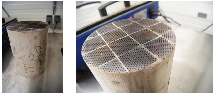
Figure 1: A deinstalled DPF, in this case originating from a Citroen C4 (left). Whereas DPF's vary in size and shape, the height of this DPF is approximately 20 cm; its radius is about 10 cm. A DPF is installed in the exhaust pipe of the vehicle. The zoom-in at the right clearly shows the channels designed to trap the particles.
