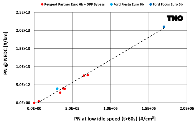
Figuur 2: PN emissions at low idle speed and NEDC tests of 3 different diesel vehicles with (cracked) DPF or variable bypass.
