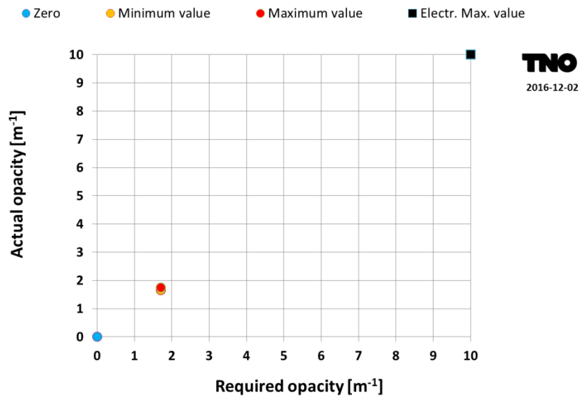
Figure 6: Specification of the accuracies of the opacimeter of UNECE R24. The accuracy of an opacimeter is only defined at a smoke emission value of 1.7 m -1 . No requirements for linearity over the total measuring range are specified.
